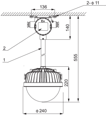
Pole mounting
