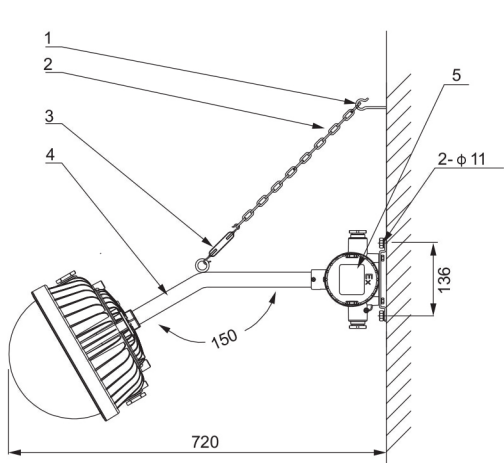
Wall mounting 150°
