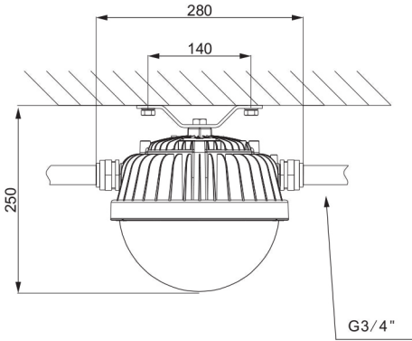
Ceiling mounting
