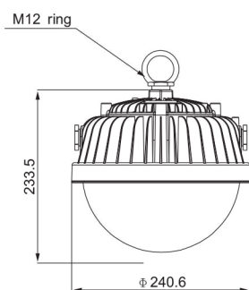
Ring mounted(Standard)
