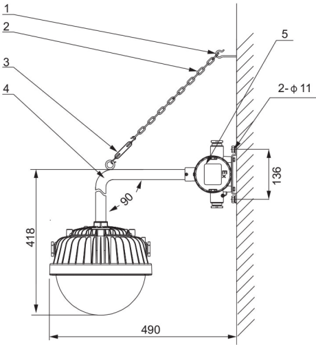
Wall mounting 90°
