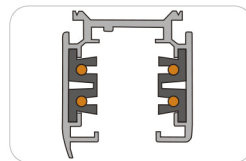
Four-line track
