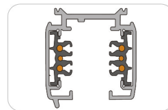
Six-line track
