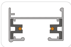
Two-line track
